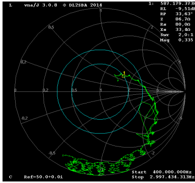
MiniVNA, LCR circuit 2 400...3000 MHz Note the graph is very noisy, and only gives an impression of impedance.
