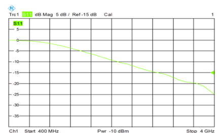
R&S 400...4000 MHz
