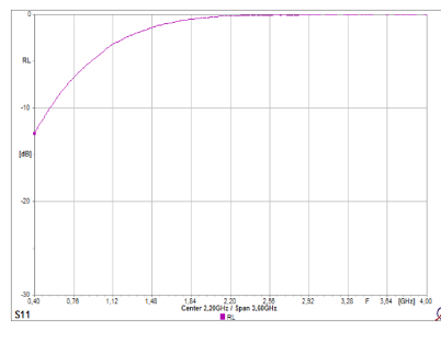
MegiQ 400...4000 MHz (-15 ... 0 dB)
