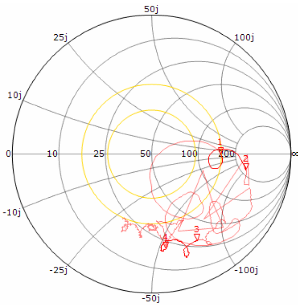
MiniVNA: A very noisy and skipping Smith Chart. It will be difficult up to impossible to read impedance of the multi resonant antenna
