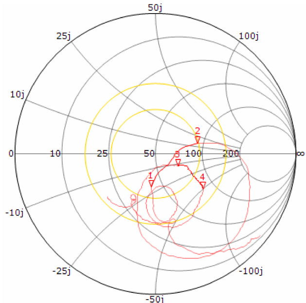
MegiQ: A clear and good to read Smith Chart.
