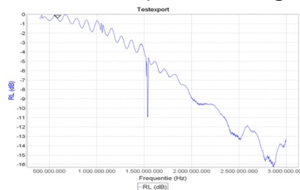
MiniVNA 1 ... 3000 MHz
