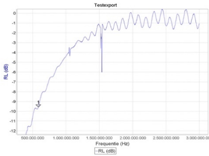
MiniVNA 1...3000 MHz (-12 ... 0 dB)
