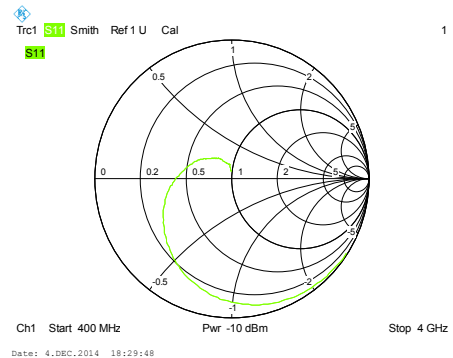
R&S, circuit 1 400...4000 MHz
