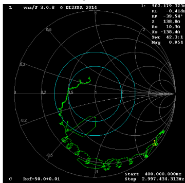
MiniVNA, circuit 1 400 ... 3000 MHz Note the graph is very noisy, and only gives an impression of impedance.
