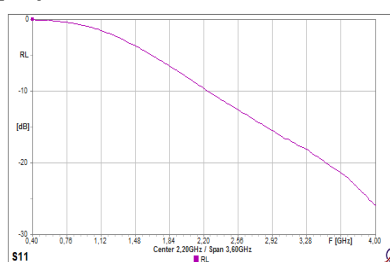
MegiQ 400...4000 MHz
